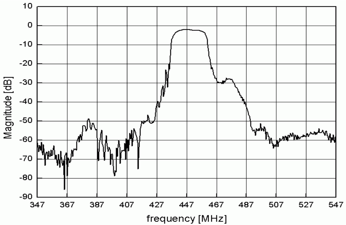
Frequency Response
